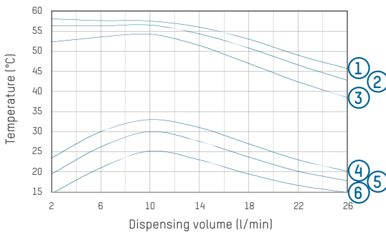
D) Domestic hot water temperature = 50 °C
