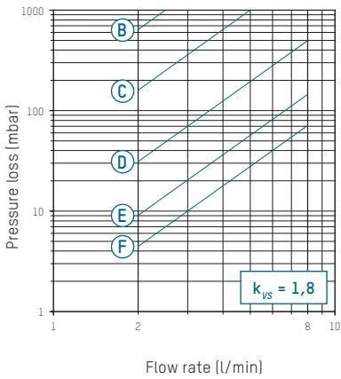
B – F Valve position
