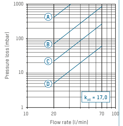
A - D Valve position
