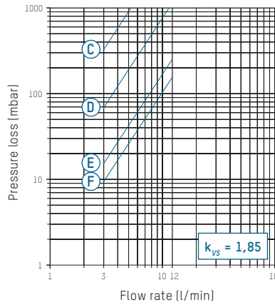
C – F Valve position
