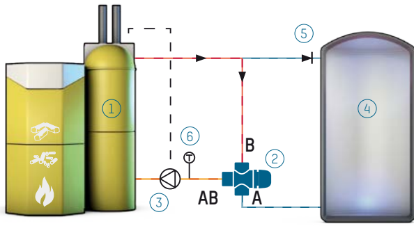
FUNCTION: MIXING
