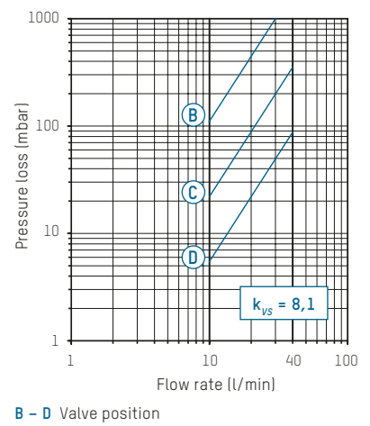
223.2480.XXX (DN 25 | 1" | 10...40 l/min)
