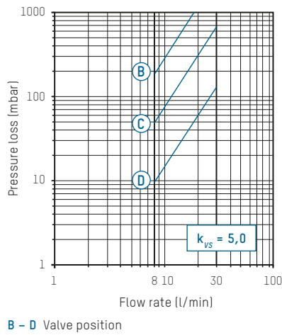
223.2383.XXX (DN 20 | 3/4" | 8...30 l/min)
