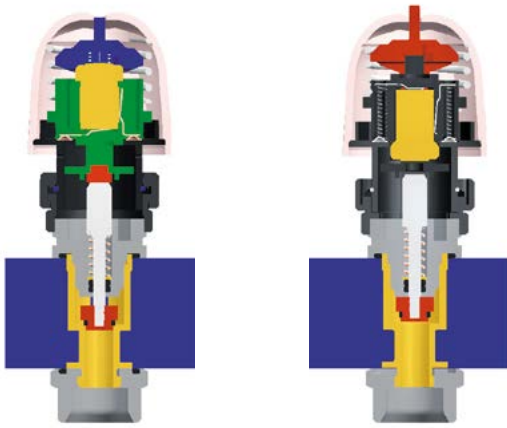
Type NC: Valve closed
