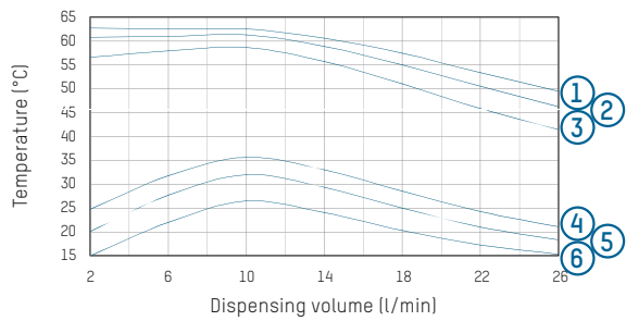
G) Domestic hot water temperature = 55 °C
