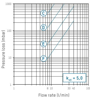
C – F Valve position
