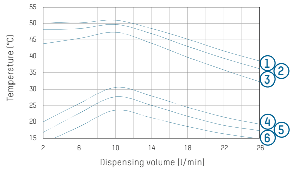
G) Domestic hot water temperature = 55 °C
