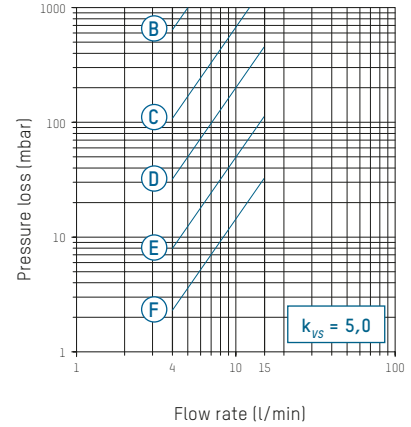
C – F Valve position
