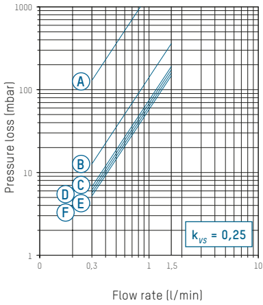
A – F Valve position
