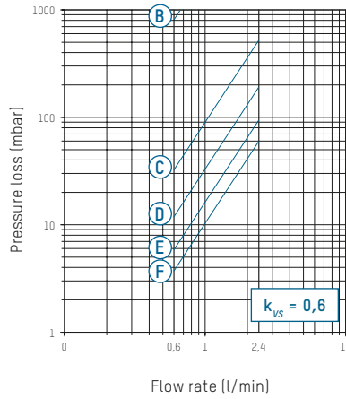
B – F Valve position
