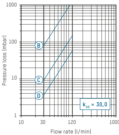
B - D Valve position
