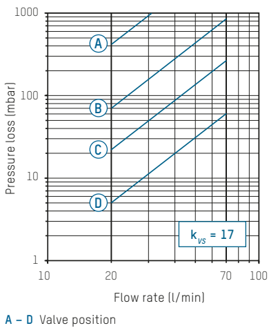
223.2580.000 (DN 32 | 1 1/4" | 20...70 l/min)
