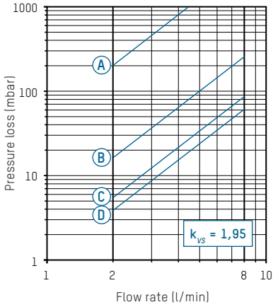
A - D Valve position
