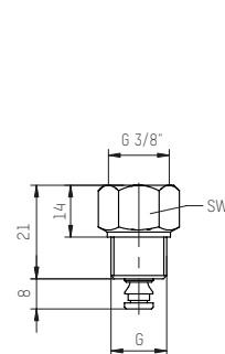
Automatic check valve DN10
