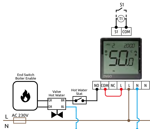
b) Connection diagram for hot water valve via hot water stat.
