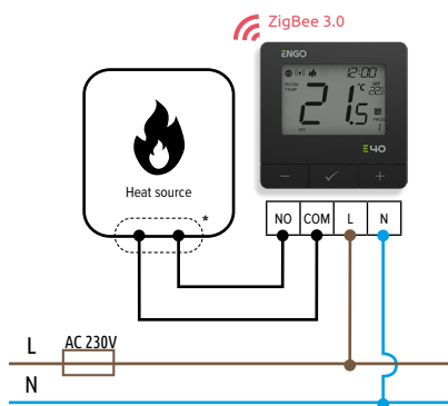
a) Connection diagram to the heat source
