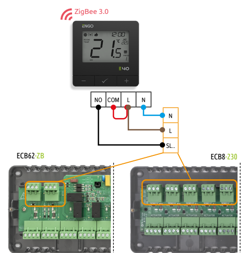
c) Connection diagram to the control strip
